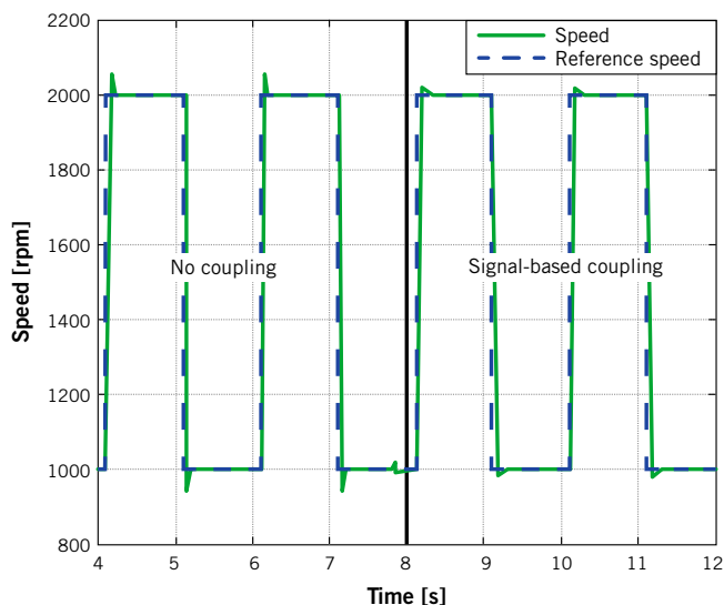
6 Comparison of measurement results with and without Acorta coupling – clear overshoot of the dyno-speed if there is no coupling (peaks in green)
